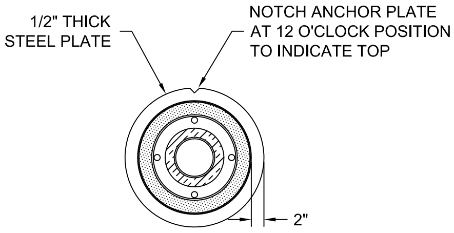
CROSS SECTION X-X ROUND ANCHOR 1/2" THICK
