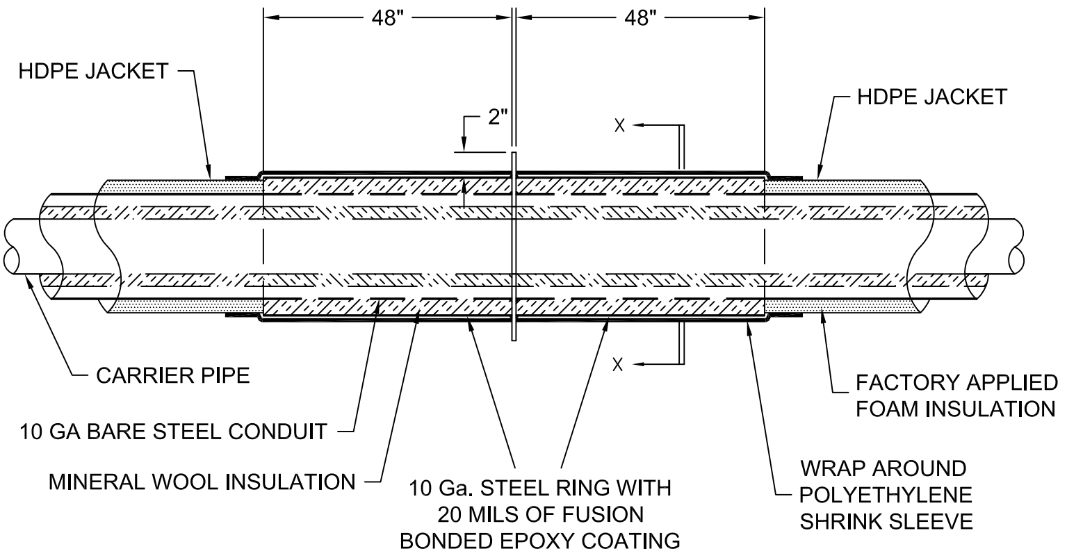
INSUL-800 ANCHOR DETAIL
