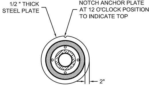
CROSS SECTION X-X ROUND ANCHOR 1/2" THICK
